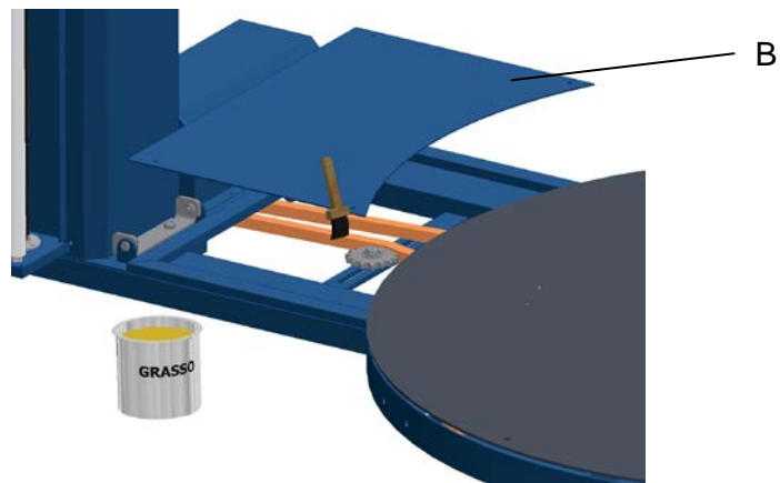
GREASING OF THE TABLE ROTATION CHAIN
